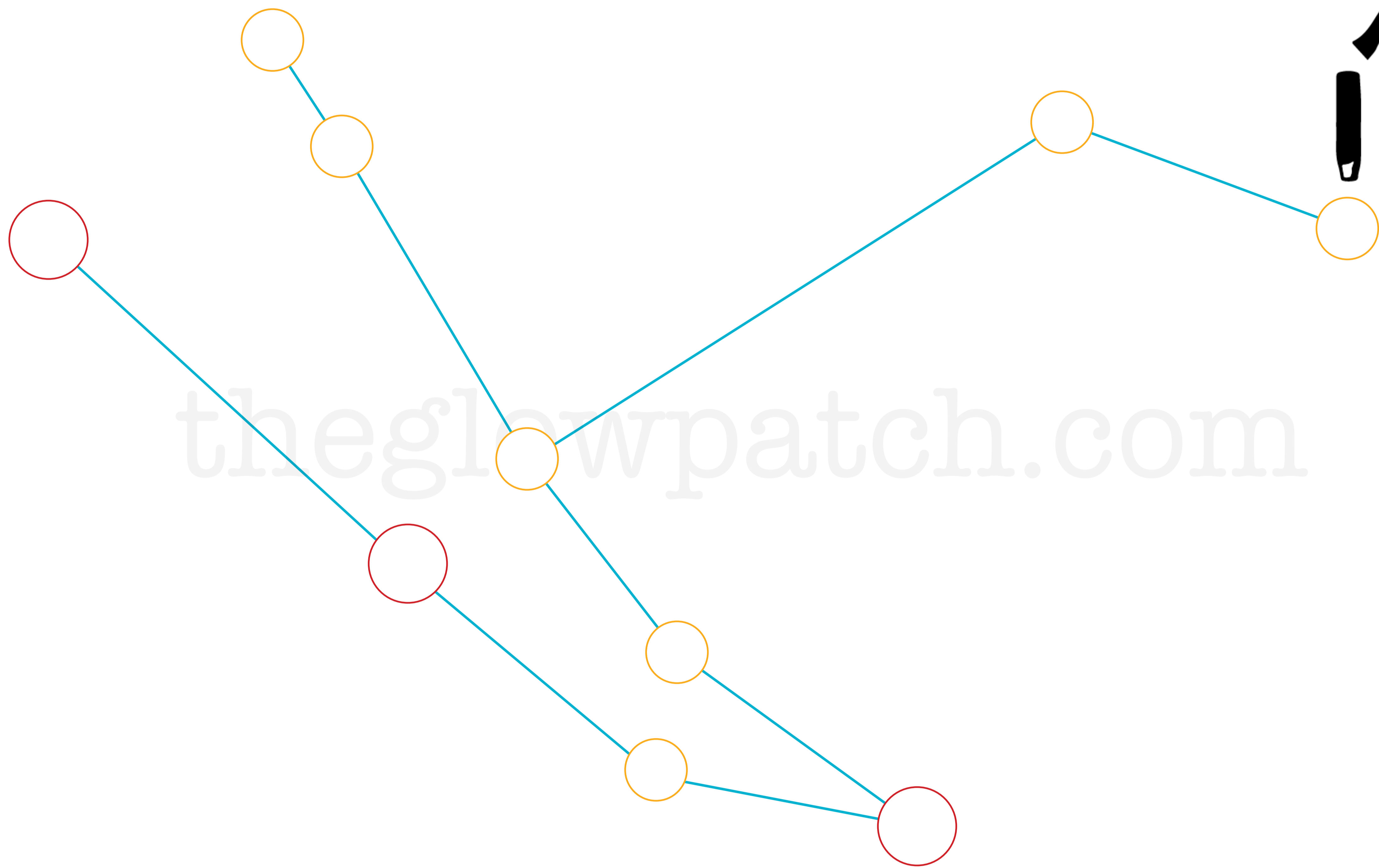
Andromeda Constellation Map
